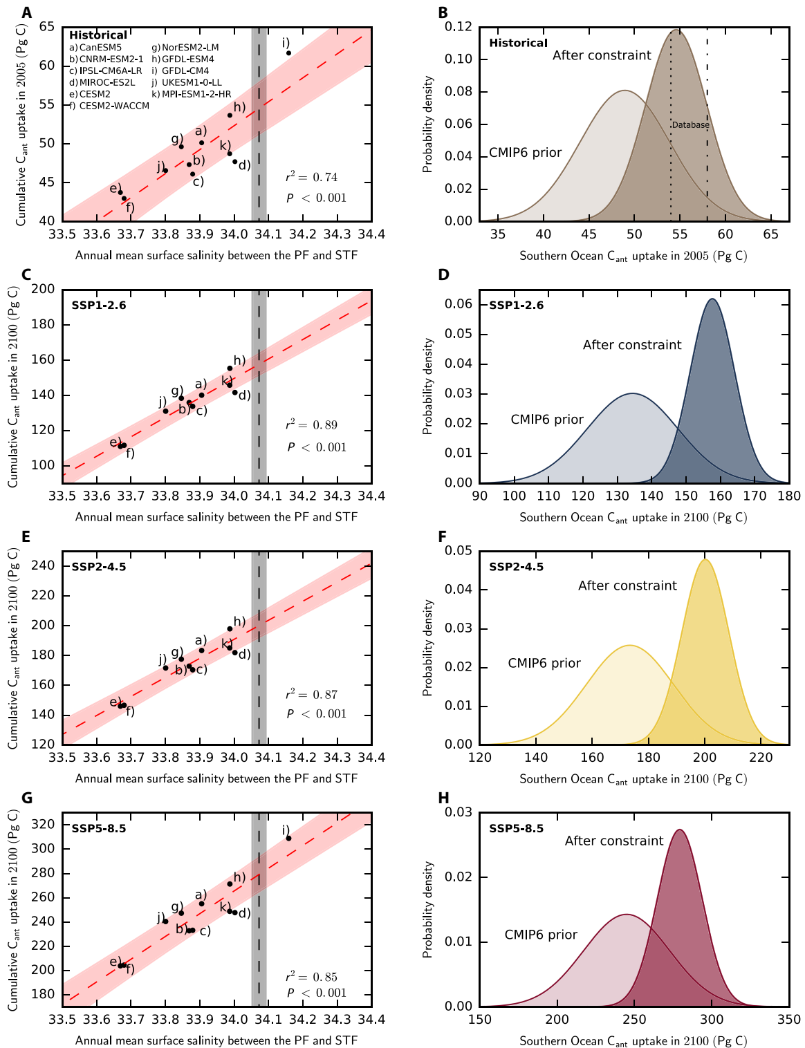
Fig. 3. Emergent constraints on the cumulative Southern Ocean C_{ant} uptake in CMIP6. The projected cumulative C_{ant} uptake in the Southern Ocean south of 30^{\circ}S across the CMIP6 model ensemble for (A) the historical period from 1850 to 2005, and the historical and future period from 1850 to 2100 under (C) SSP1-2.6, (E) SSP2-4.5, and (G) SSP5-8.5 against the present-day (1986–2005) mean sea surface salinity between the PF and STF. Linear regression fits (red dashed lines) and the associated 68% prediction intervals are shown in (A), (C), (E), and (G), as are observation-based estimates of present-day annual sea surface density between the PF and STF (black dashed lines) with the associated uncertainty (black shaded area). Probability density functions for the cumulative Southern Ocean C_{ant} uptake from (B) 1850 to 2005 and from 1850 to 2100 under (D) SSP1-2.6, (F) SSP2-4.5, and (H) SSP5-8.5, before (“CIP6 prior,” transparent) and after (“after constraint,” opaque) the emergent constraint is applied. Data-based estimates are shown in (B) as dash-dotted (5, 7) and dotted (8) lines and are scaled to the same definition of C_{ant} as the models (see Materials and Methods).
